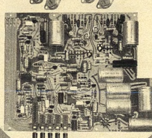
Stereomodul**)
